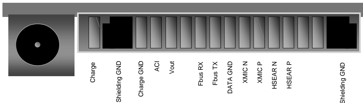
Figure 15: Pop Port System Connector
