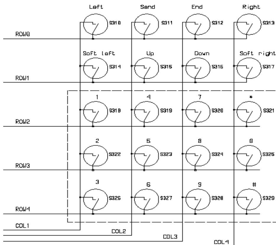
Figure 13: RH-19 keypad
