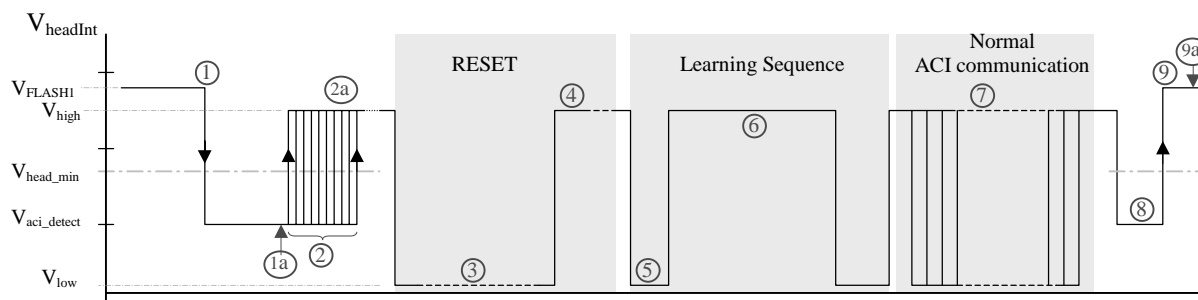
Figure 17: ACI communication
