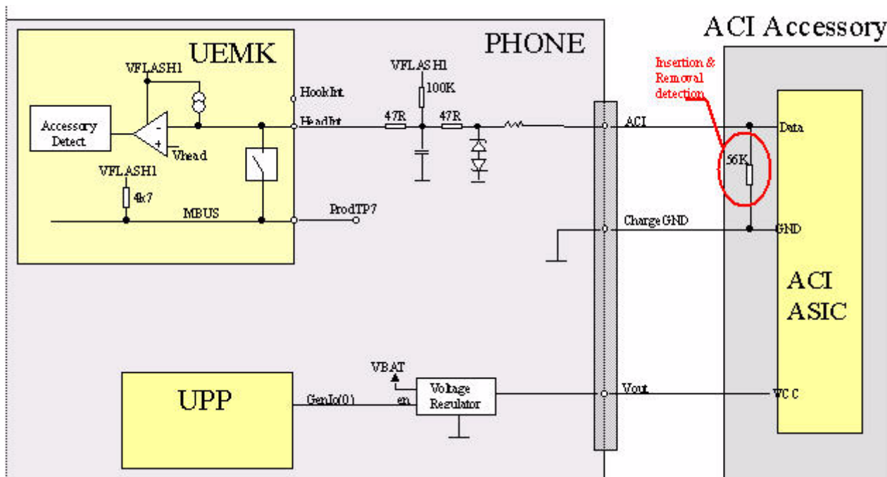
Figure 16: Principle schematics of ACI Accessory and engine
