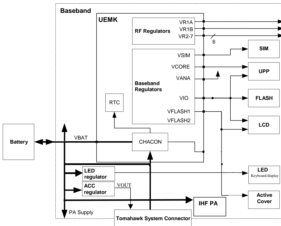
Figure 3: Baseband power distribution
