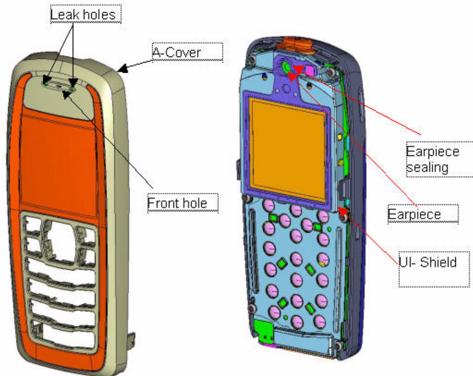
Figure 6: Earpiece implementation
