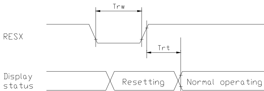
Figure 11: Reset timing
